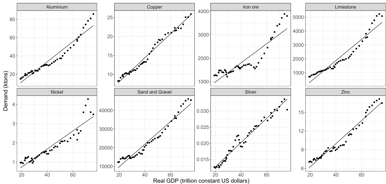
Fig. F.1. Examples for 8 main minerals of the linear regressions conducted to determine the mineral requirements of the rest of the economy (Eq. 3). These 8 minerals always account for 85% of the final energy consumption of extraction, for the subset of minerals which mineral requirements by the rest of the economy are determined with a linear regression.
