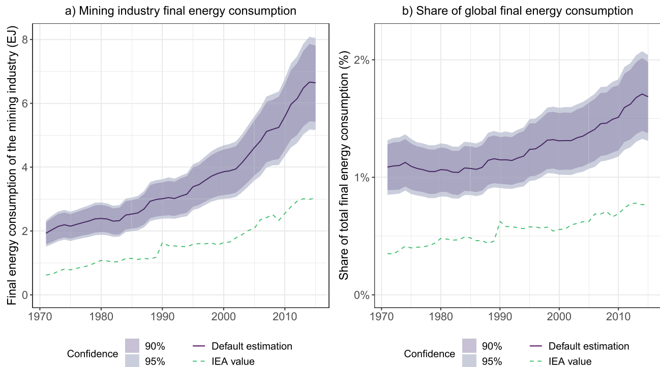
Fig. 4. Final energy consumption of the mining industry (left), and share of global final energy consumption consumed by the mining industry (right). Note that calculated values account for both direct and indirect energy, while the IEA's accounting method only includes direct energy.
