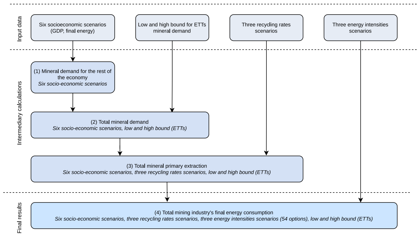
Fig. 2. Workflow for constructing future pathways of the mining industry's global final energy consumption, and possible combinations of socioeconomic scenario, recycling rates scenario, mining energy intensities scenario, and mineral requirements for ETTs. ETTs: Energy Transition Technologies.
