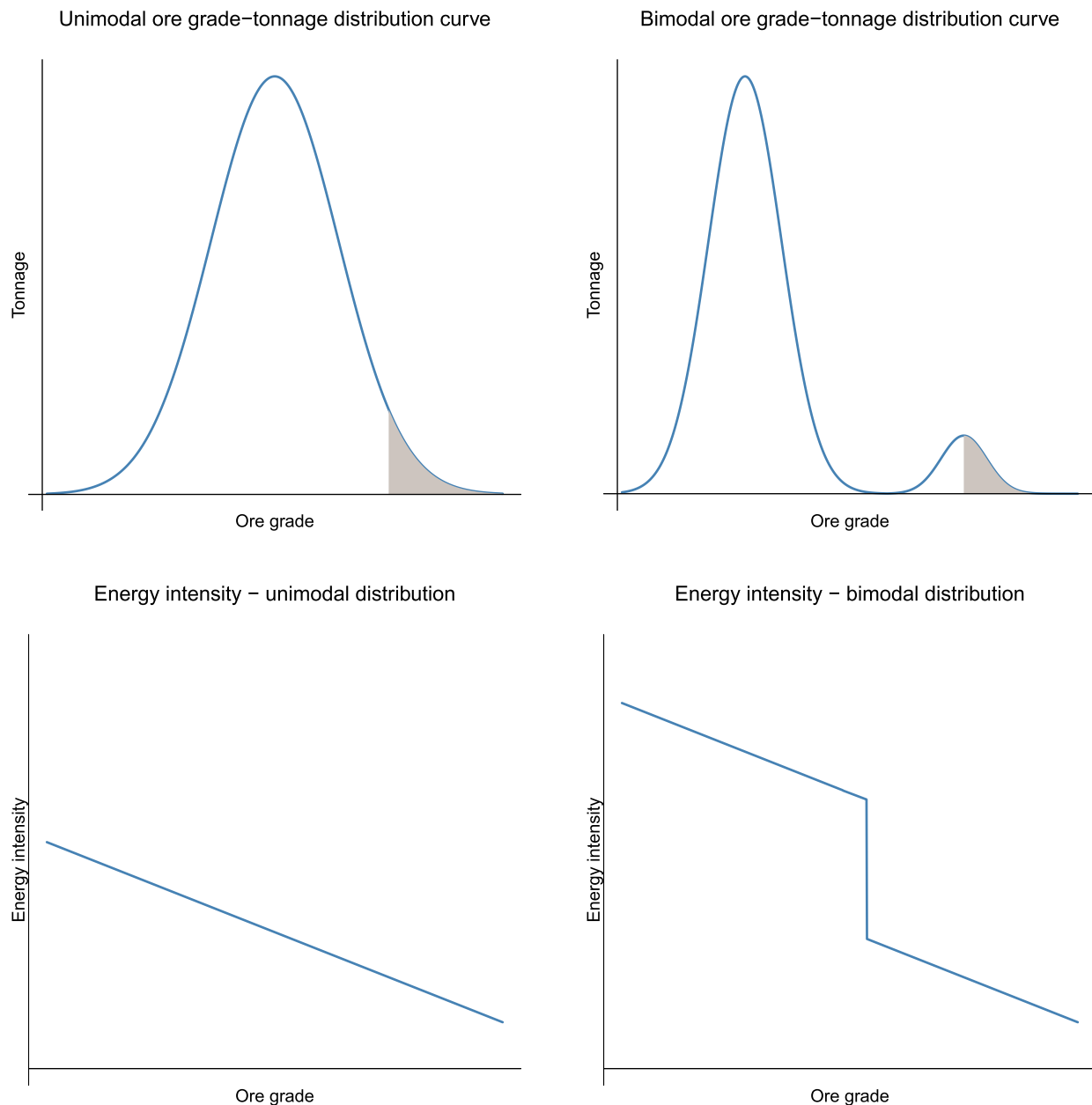
Fig. D.1. Unimodal and bimodal ore grade-tonnage distribution curves, as well as implications of each distribution in terms of evolution of energy intensities as function of ore grades. The grey area corresponds to the tonnage extracted to date.
