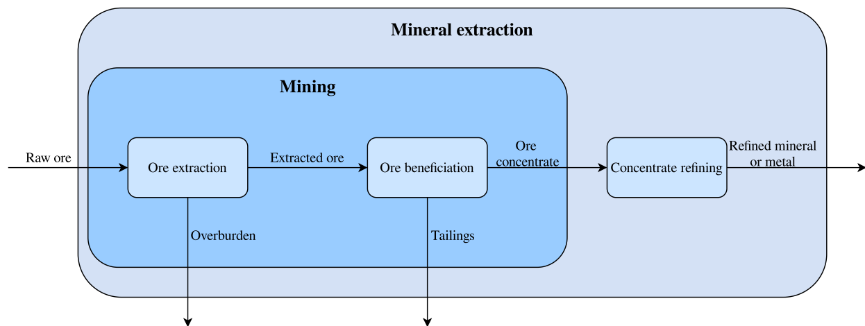
Fig. 1. Graphical representation of the mineral extraction process. The mining activities cover the ore extraction and ore beneficiation steps, while the refining process, mostly relevant for metals, belongs to the metallurgical industry. Energy intensities only refer to the ore extraction and ore beneficiation stages in this paper.
