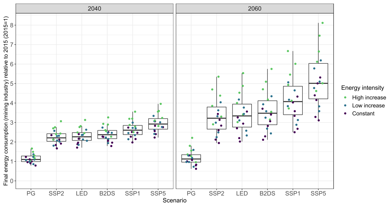
Fig. 6. Final energy consumption of the mining industry in 2060 relative to 2015, for each different socio-economic, recycling rate, energy intensity, and renewable energy scenario. (2015=1.) Points with the same colour and shape correspond to the high and low range of mineral demand for the Energy Transition Technologies, with the same recycling rate and energy intensity scenarios. Energy intensity refers to the \alpha variable.
